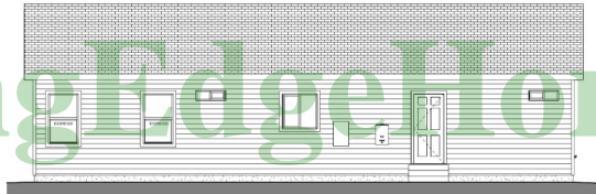
③ REAR ELEVATION 1/4" = 1'-0"
