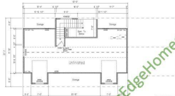
UPPER LEVEL FLOORPLAN 1164 SQ. FT. OPTIONAL FOUR BED ROOM AREA
